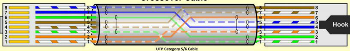
Crossover Cable
